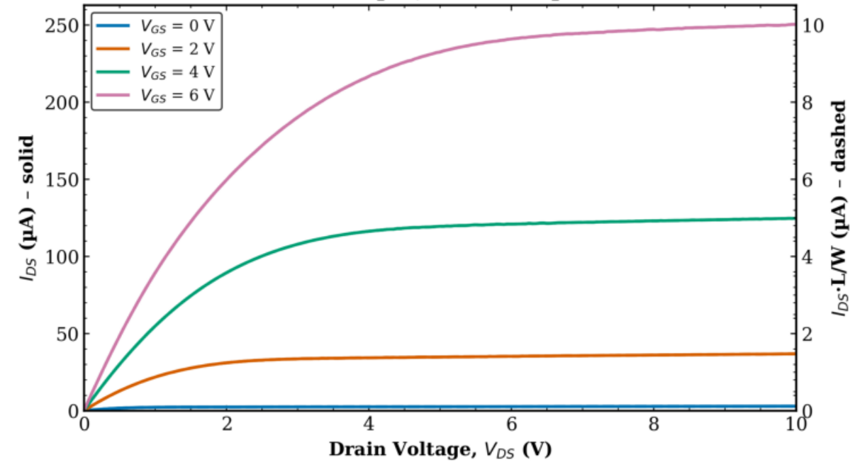
TFT1 Transistor 2 L = 20 \mu\text{m} , W = 500 \mu\text{m}
