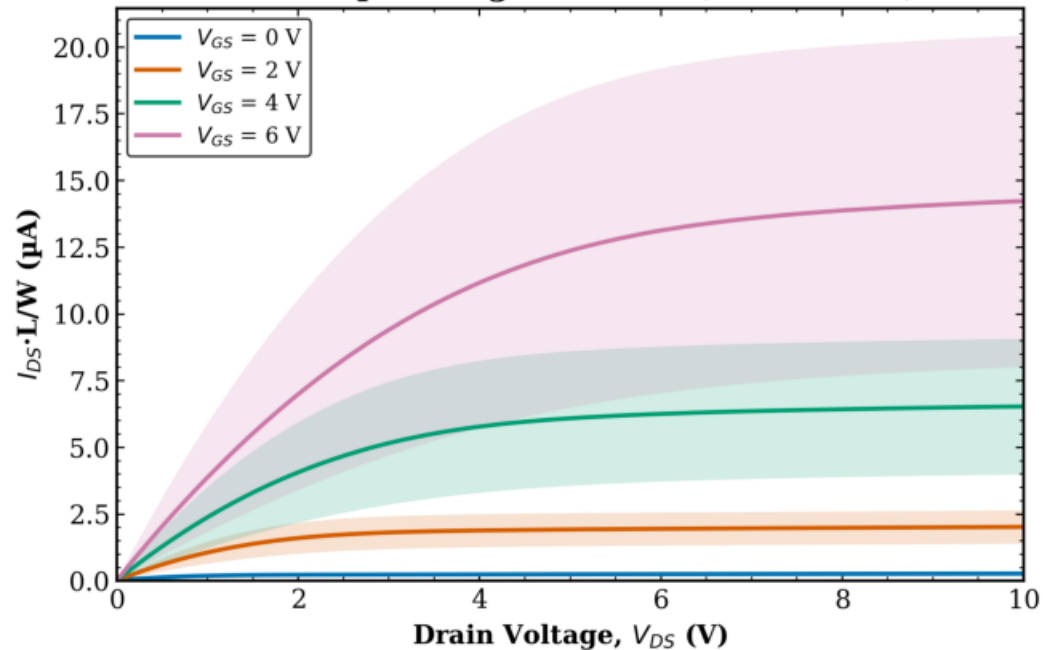
TFT1 Transistor 2 W = 10 \mu\text{m} - avg over all L (mean \pm std)
