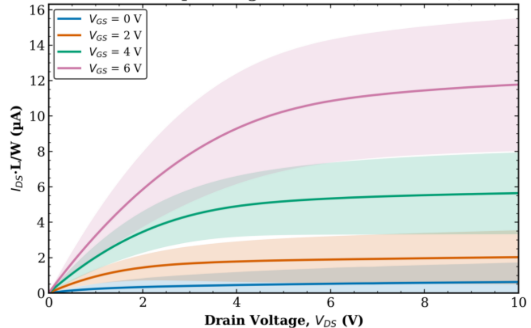
TFT1 Transistor 2 W = 100 \mu\text{m} - avg over all L (mean \pm std)
