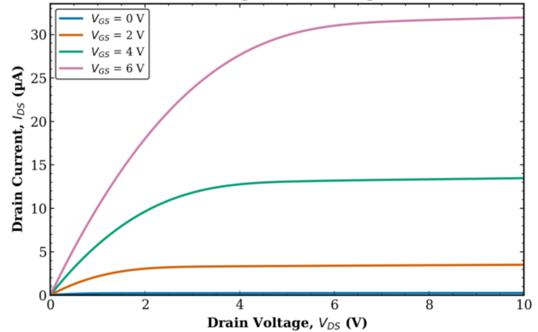
TFT1 Transistor 2 L = 40 \mu\text{m} , W = 100 \mu\text{m}
