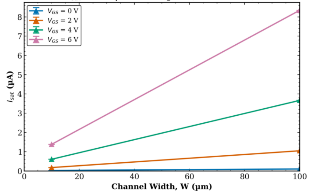
TFT1 Transistor 2 I_{sat} vs W | L = 160 \mu\text{m} (mean \pm std)
