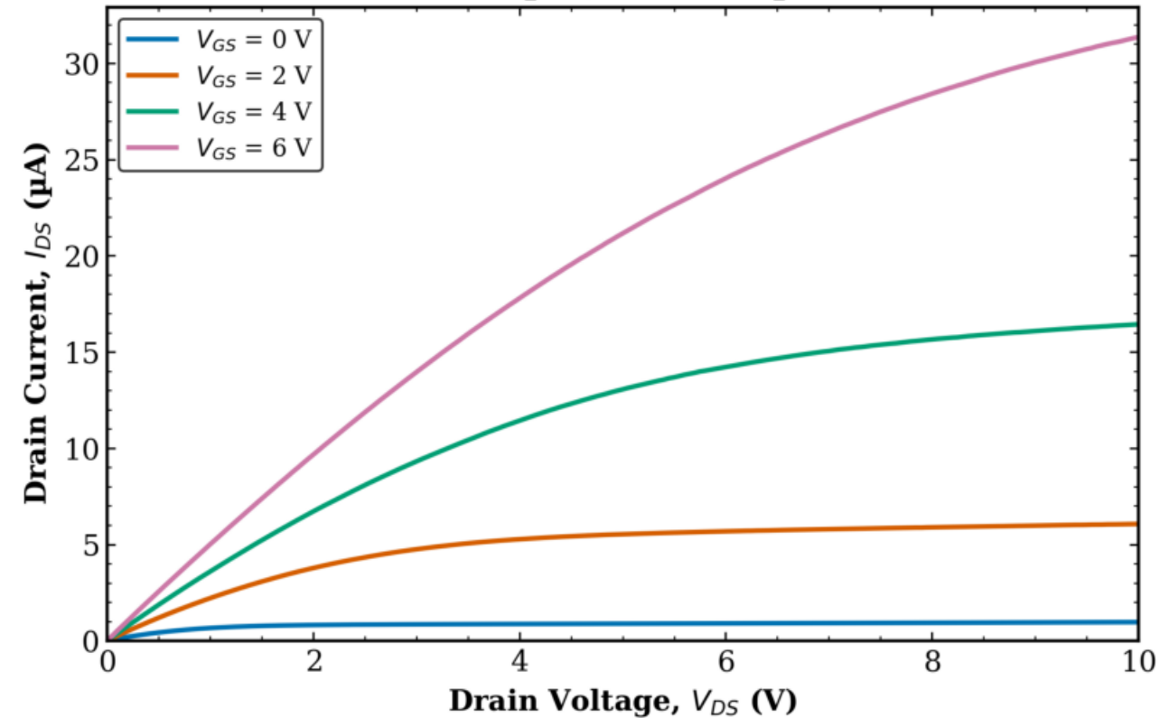
TFT1 Transistor 2 L = 8 \mu\text{m} , W = 50 \mu\text{m}
