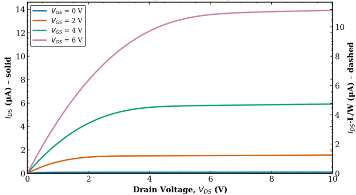
TFT1 Transistor 2 L = 80 \mu\text{m} , W = 100 \mu\text{m}
