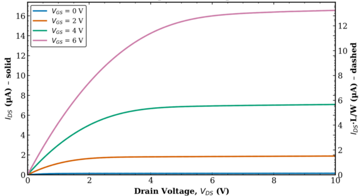
TFT1 Transistor 2 L = 40 \mu\text{m} , W = 50 \mu\text{m}
