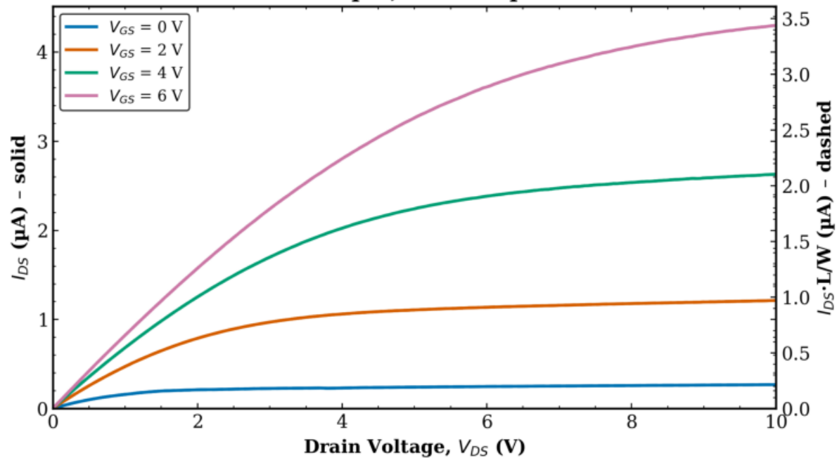
TFT1 Transistor 2 L = 8 \mu\text{m} , W = 10 \mu\text{m}
