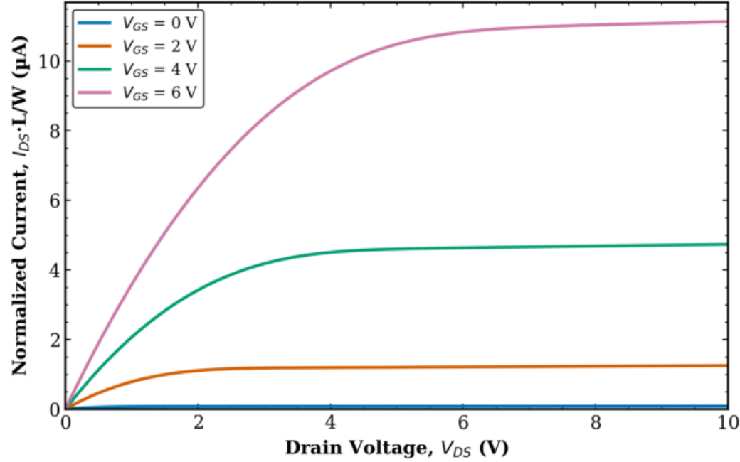
TFT1 Transistor 2 L = 80 \mu\text{m} , W = 100 \mu\text{m} (normalized)
