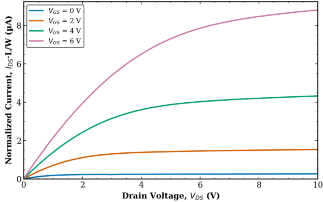
TFT1 Transistor 2 L = 10 \mu\text{m} , W = 10 \mu\text{m} (normalized)
