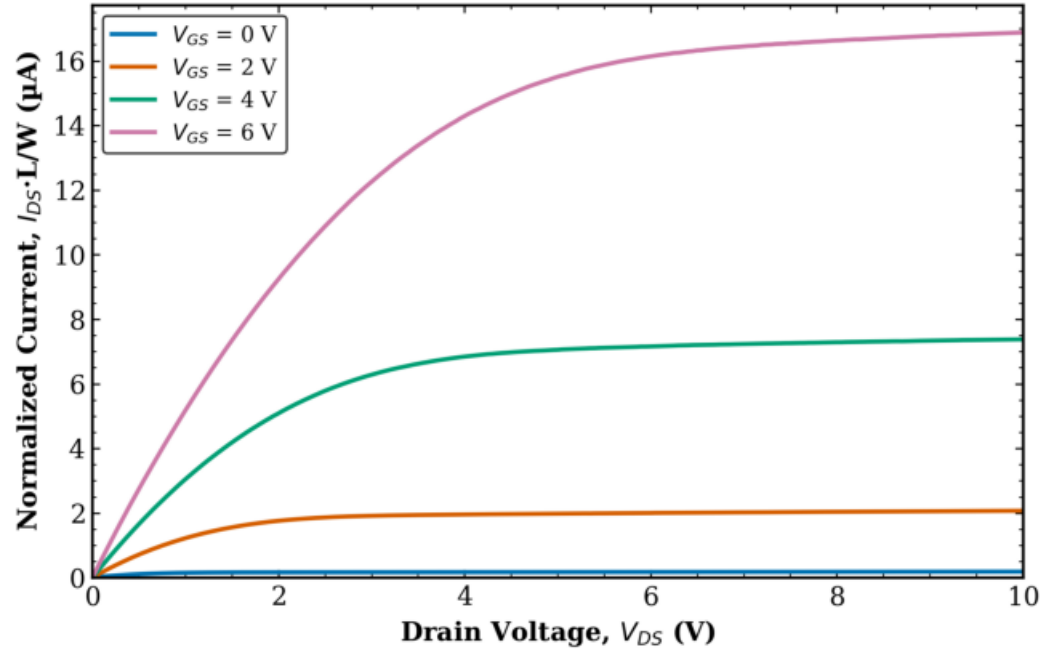
TFT1 Transistor 2 L = 40 \mu\text{m} , W = 10 \mu\text{m} (normalized)
