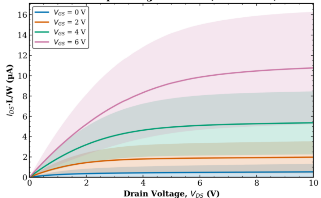
TFT1 Transistor 2 W = 50 \mu\text{m} - avg over all L (mean \pm std)
