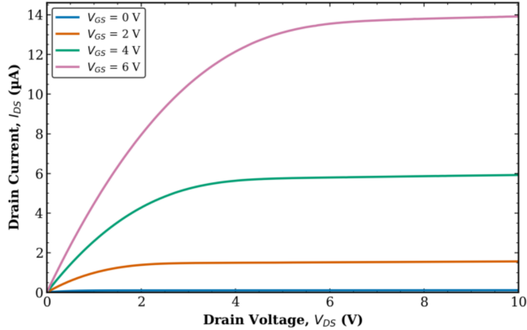
TFT1 Transistor 2 L = 80 \mu\text{m} , W = 100 \mu\text{m}
