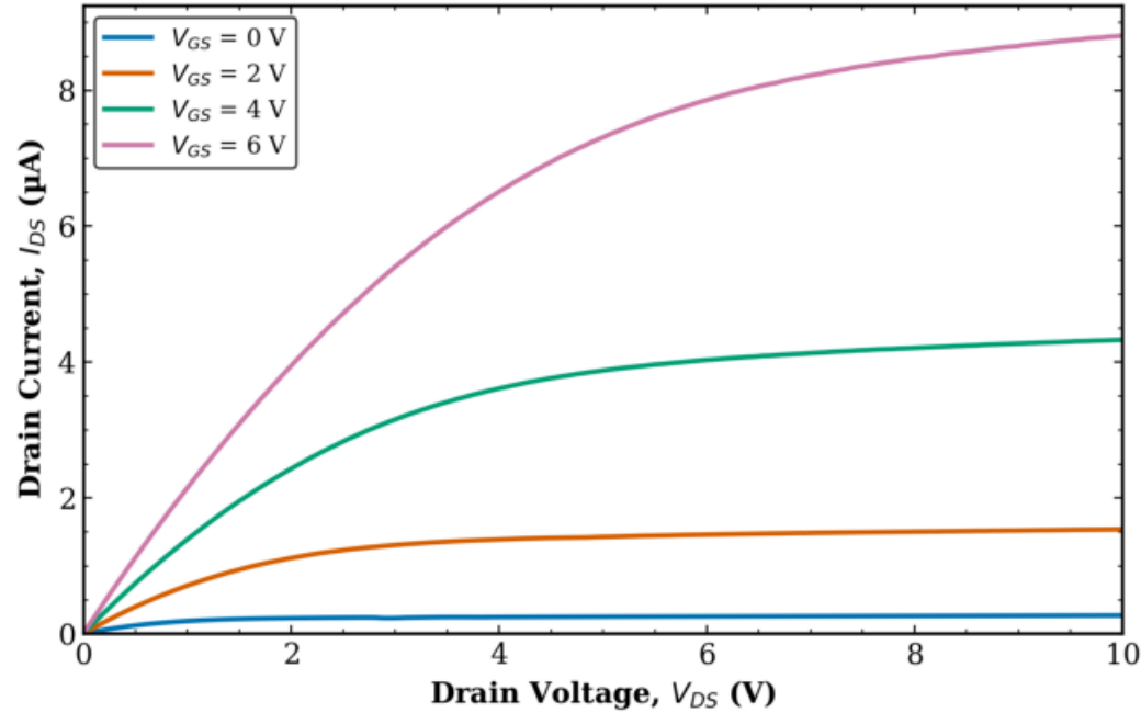
TFT1 Transistor 2 L = 10 \mu\text{m} , W = 10 \mu\text{m}
