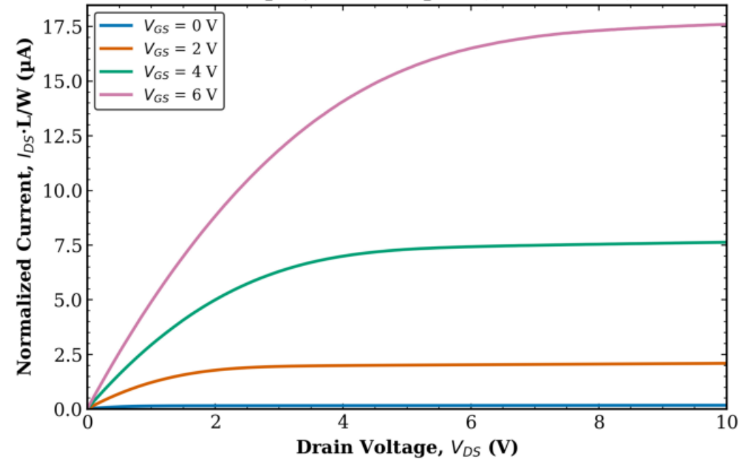
TFT1 Transistor 2 L = 80 \mu\text{m} , W = 10 \mu\text{m} (normalized)
