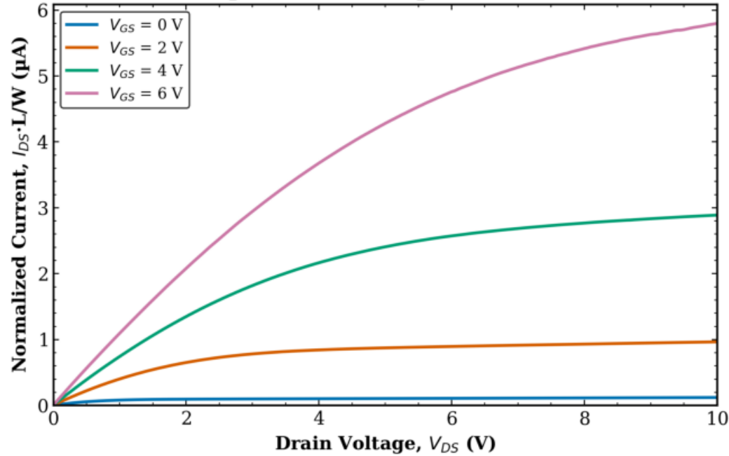
TFT1 Transistor 2 L = 10 \mu\text{m} , W = 1000 \mu\text{m} (normalized)
