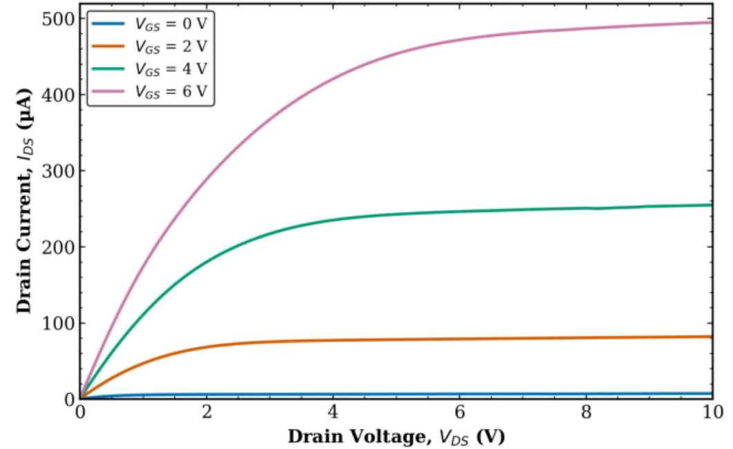
TFT1 Transistor 2 L = 20 \mu\text{m} , W = 1000 \mu\text{m}
