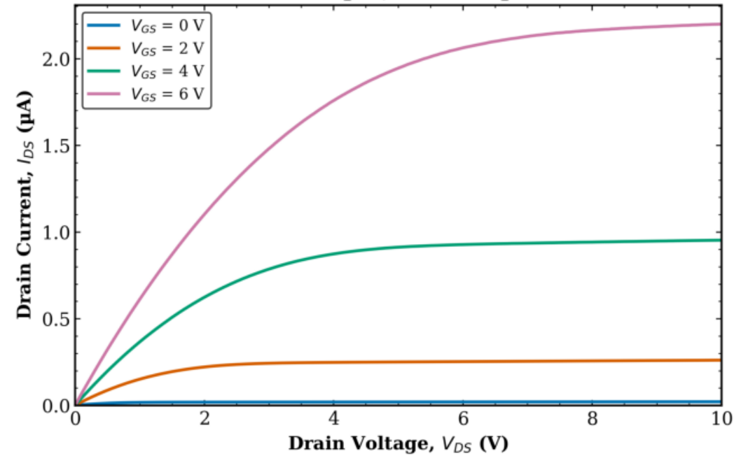
TFT1 Transistor 2 L = 80 \mu\text{m} , W = 10 \mu\text{m}
