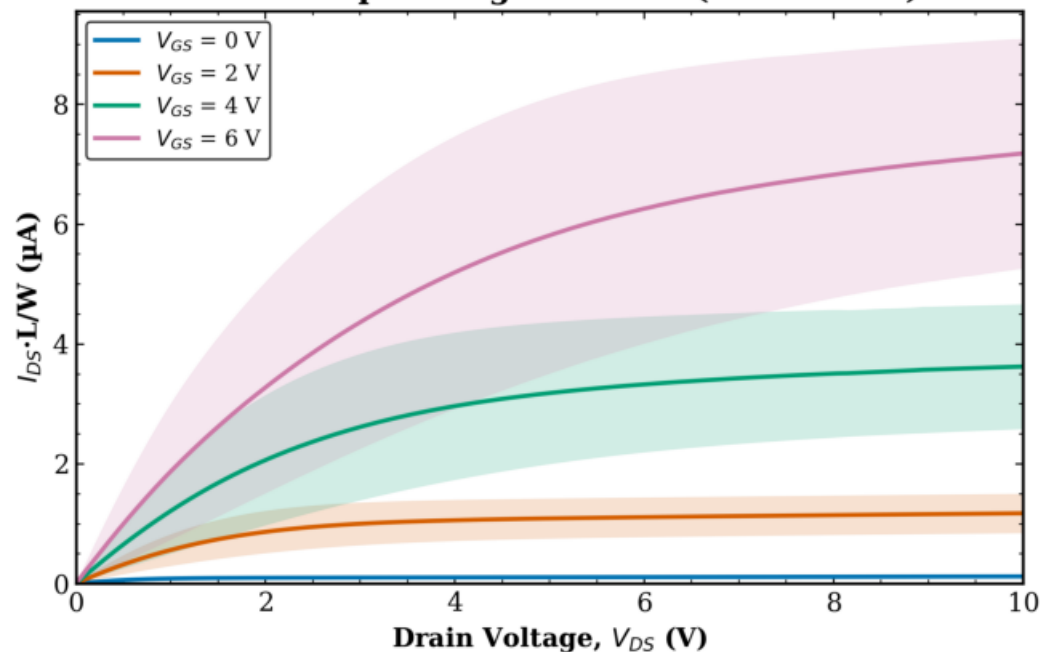
TFT1 Transistor 2 W = 1000 \mu\text{m} - avg over all L (mean \pm std)
