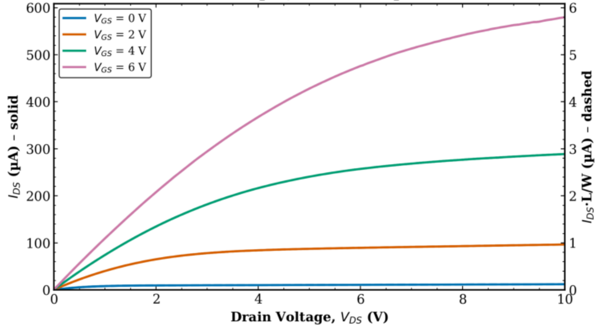
TFT1 Transistor 2 L = 10 \mu\text{m} , W = 1000 \mu\text{m}
