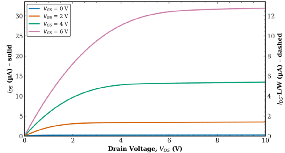
TFT1 Transistor 2 L = 40 \mu\text{m} , W = 100 \mu\text{m}
