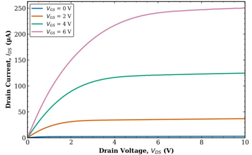
TFT1 Transistor 2 L = 20 \mu\text{m} , W = 500 \mu\text{m}
