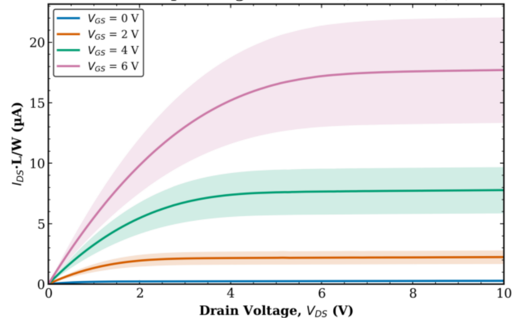
TFT1 Transistor 2 L = 160 \mu\text{m} - avg over all W (mean \pm std)
