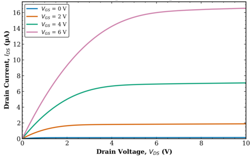
TFT1 Transistor 2 L = 40 \mu\text{m} , W = 50 \mu\text{m}
