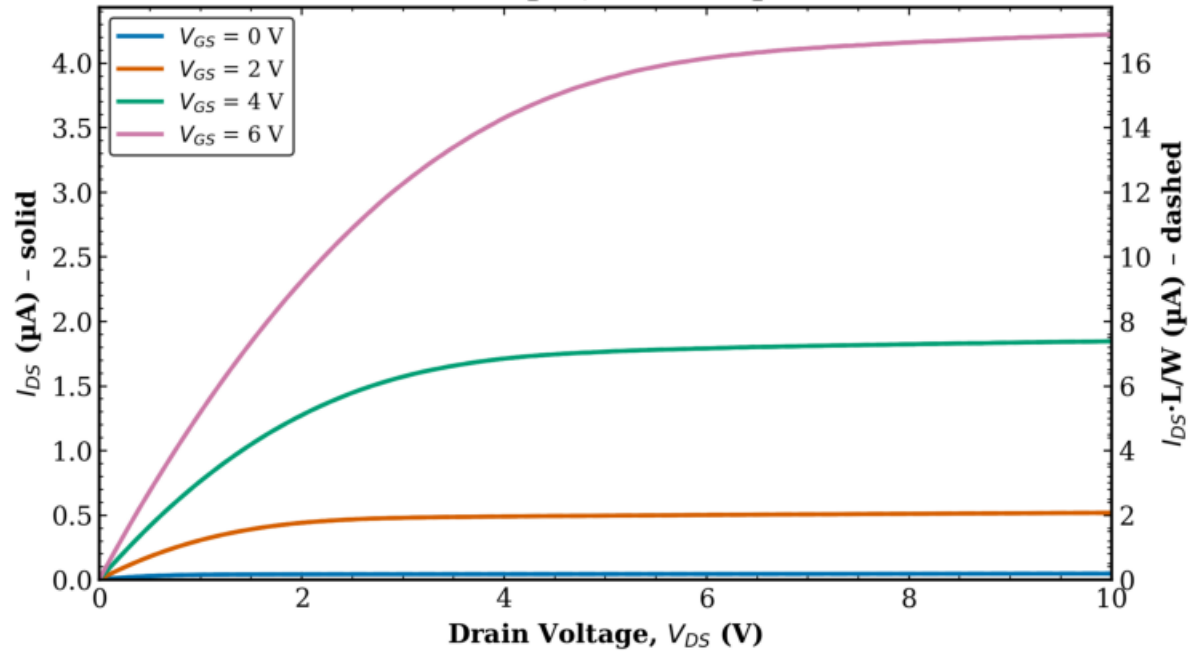
TFT1 Transistor 2 L = 40 \mu\text{m} , W = 10 \mu\text{m}
