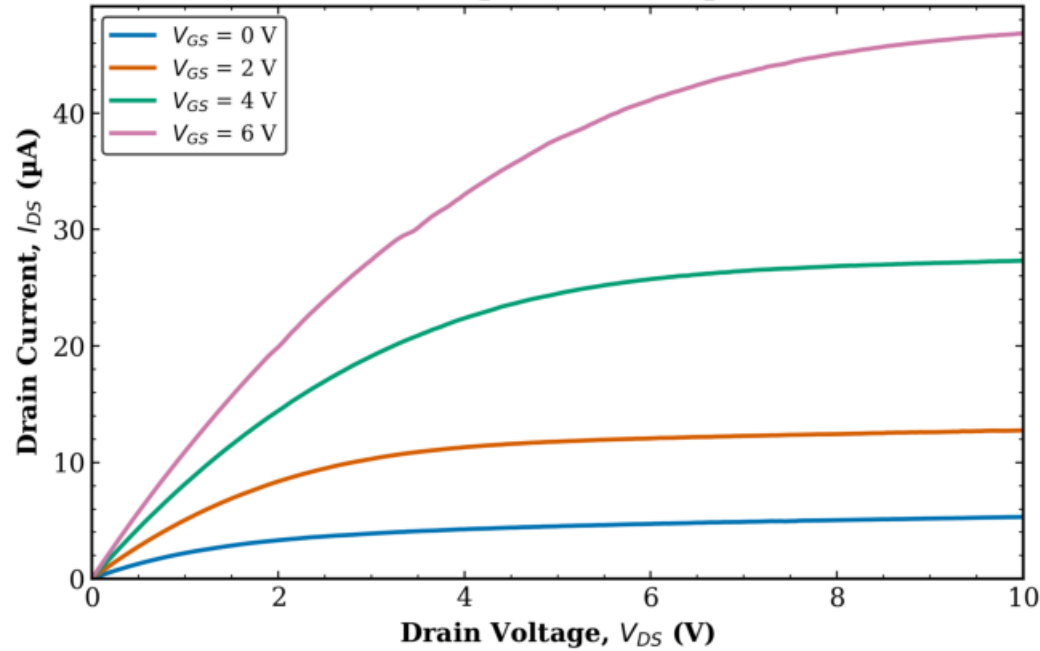
TFT1 Transistor 2 L = 20 \mu\text{m} , W = 50 \mu\text{m}
