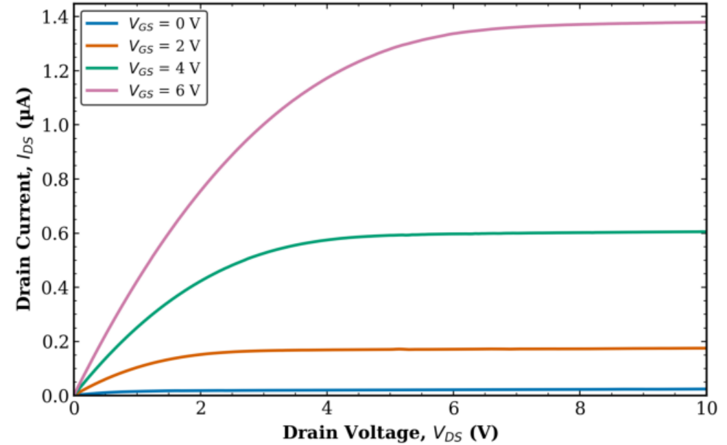
TFT1 Transistor 2 L = 160 \mu\text{m} , W = 10 \mu\text{m}
