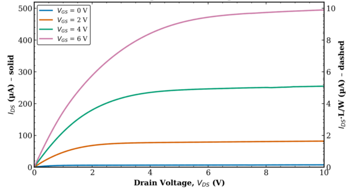
TFT1 Transistor 2 L = 20 \mu\text{m} , W = 1000 \mu\text{m}
