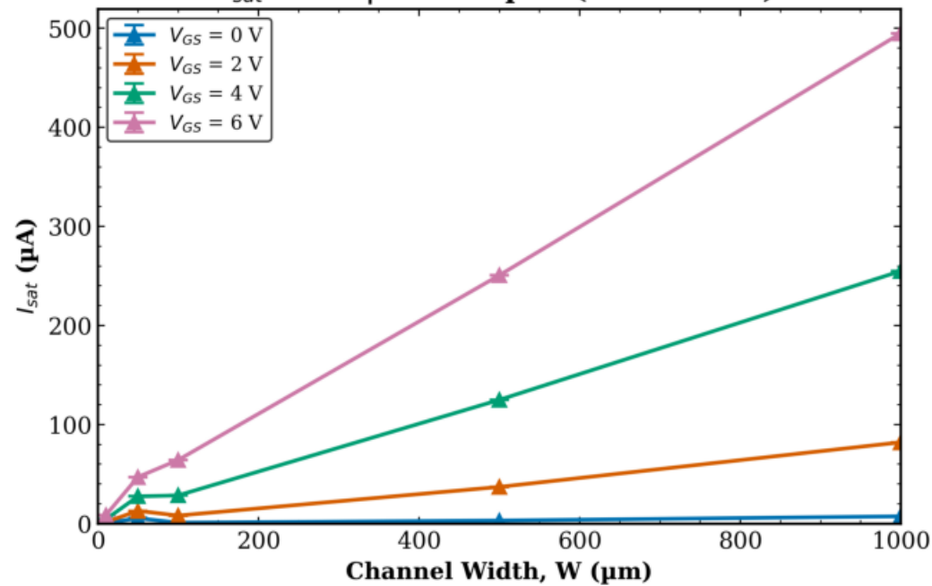
TFT1 Transistor 2 I_{sat} vs W | L = 20 \mu\text{m} (mean \pm std)
