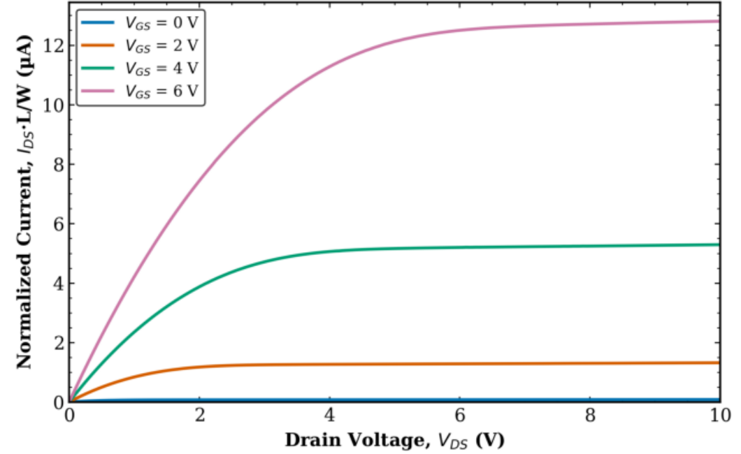
TFT1 Transistor 2 L = 80 \mu\text{m} , W = 50 \mu\text{m} (normalized)
