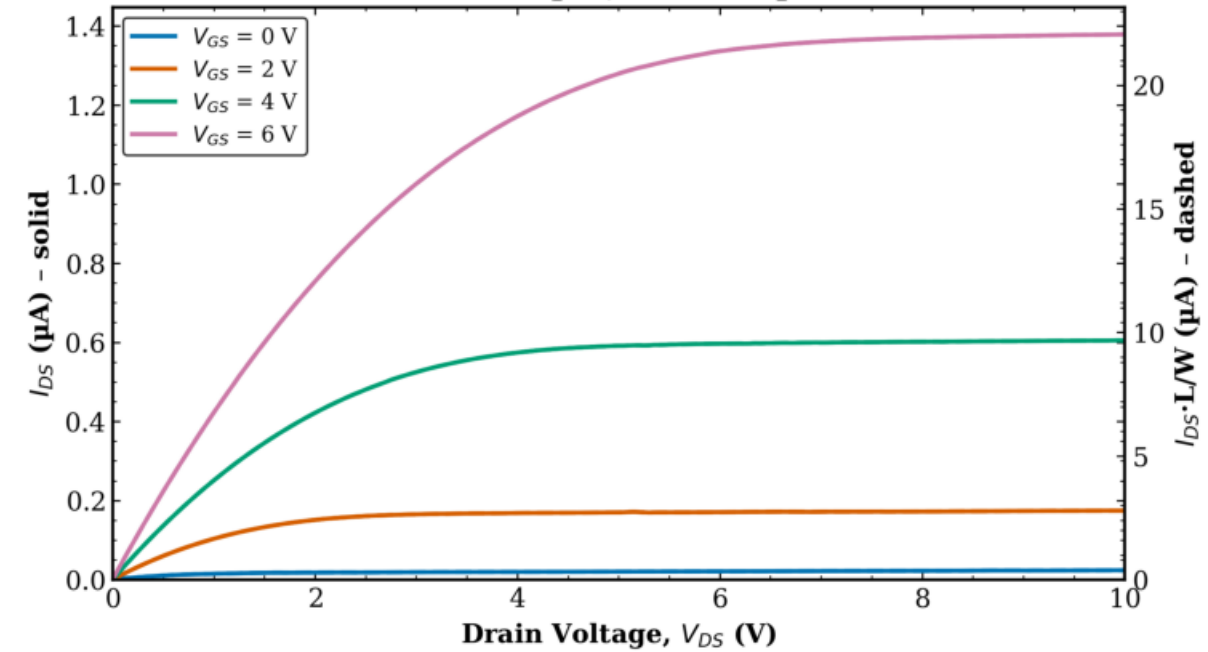
TFT1 Transistor 2 L = 160 \mu\text{m} , W = 10 \mu\text{m}
