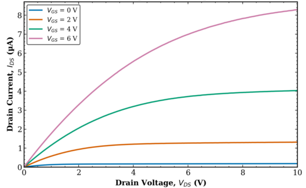
TFT1 Transistor 2 L = 20 \mu\text{m} , W = 10 \mu\text{m}
