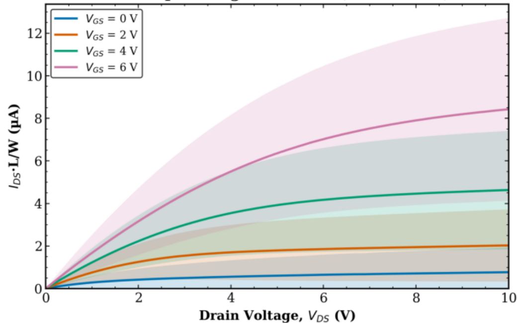
TFT1 Transistor 2 L = 10 \mu\text{m} - avg over all W (mean \pm std)
