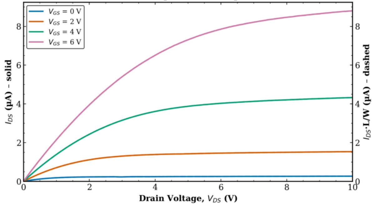
TFT1 Transistor 2 L = 10 \mu\text{m} , W = 10 \mu\text{m}
