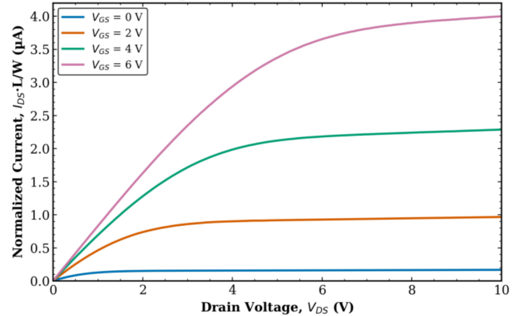
TFT1 Transistor 2 L = 10 \mu\text{m} , W = 50 \mu\text{m} (normalized)
