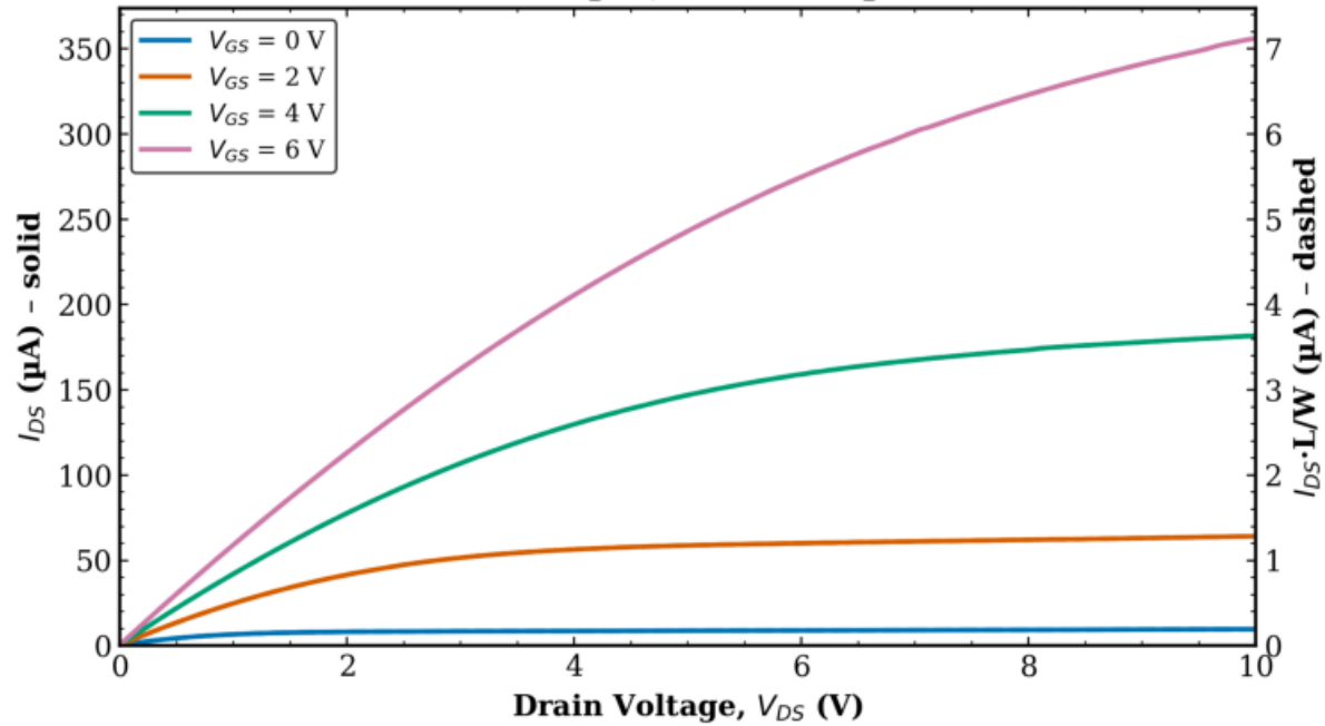
TFT1 Transistor 2 L = 10 \mu\text{m} , W = 500 \mu\text{m}
