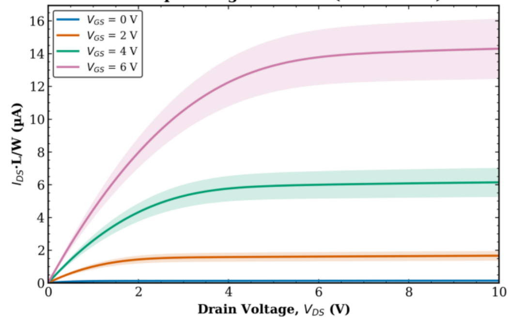
TFT1 Transistor 2 L = 40 \mu\text{m} - avg over all W (mean \pm std)
