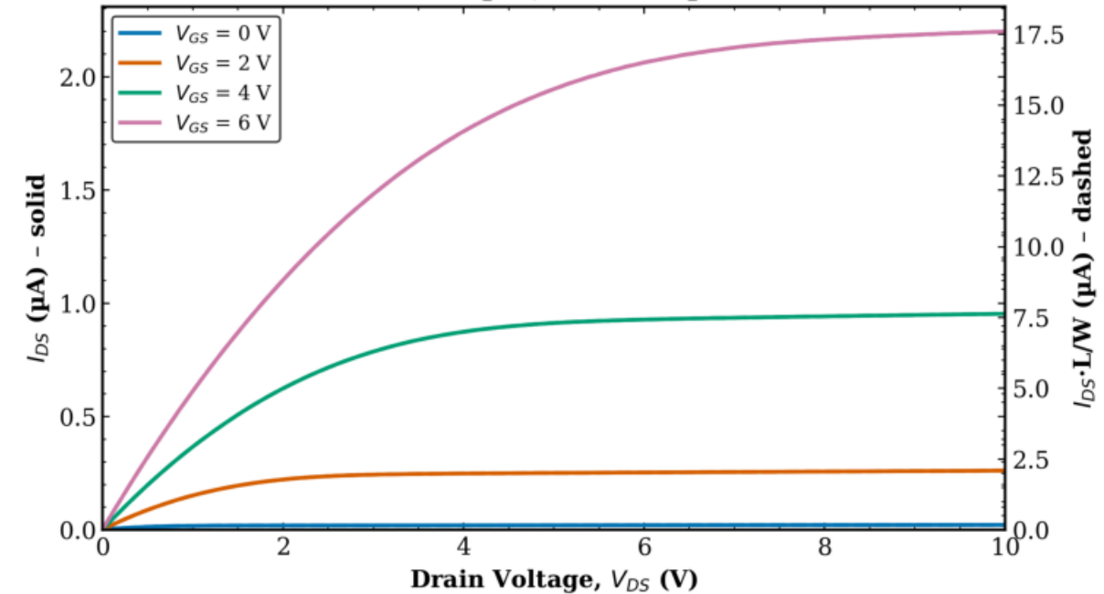
TFT1 Transistor 2 L = 80 \mu\text{m} , W = 10 \mu\text{m}
