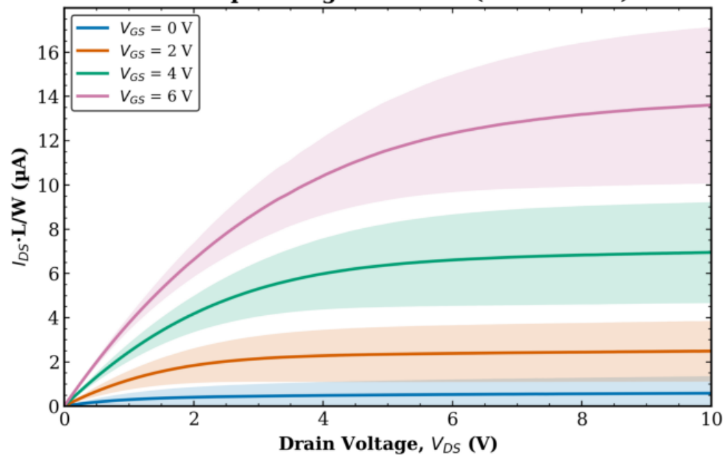
TFT1 Transistor 2 L = 20 \mu\text{m} - avg over all W (mean \pm std)
