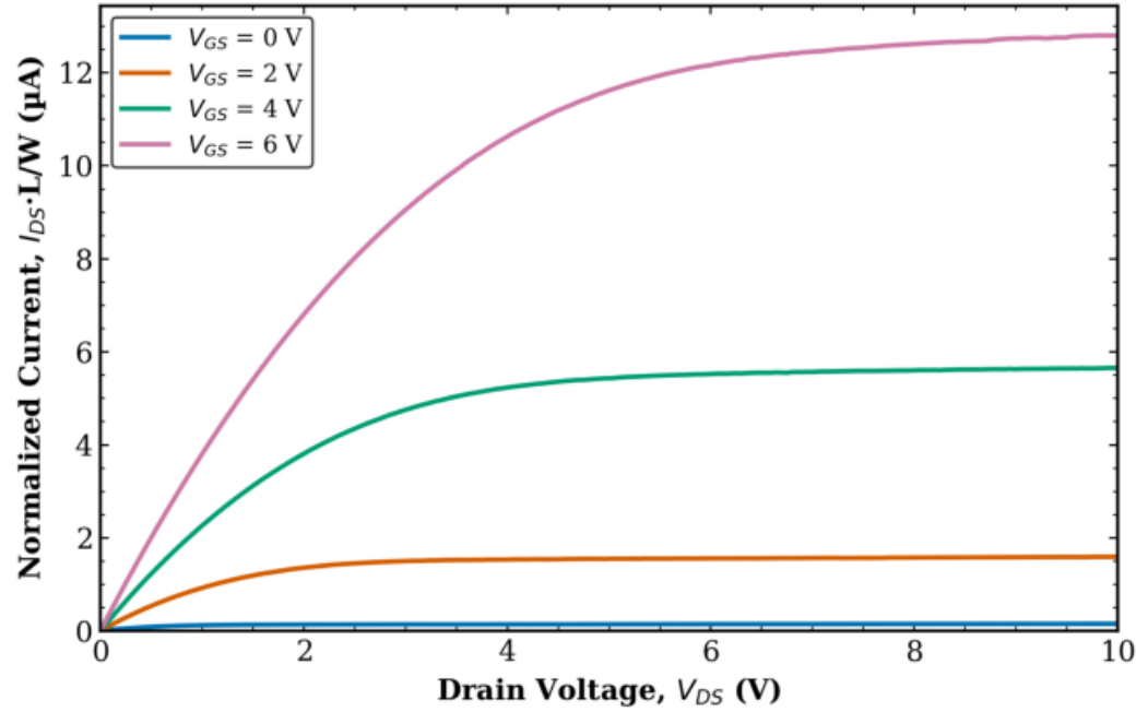
TFT1 Transistor 2 L = 20 \mu\text{m} , W = 100 \mu\text{m} (normalized)
