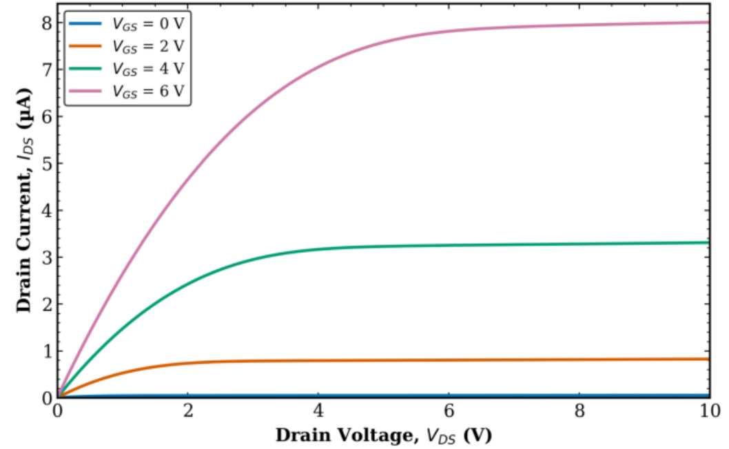
TFT1 Transistor 2 L = 80 \mu\text{m} , W = 50 \mu\text{m}
