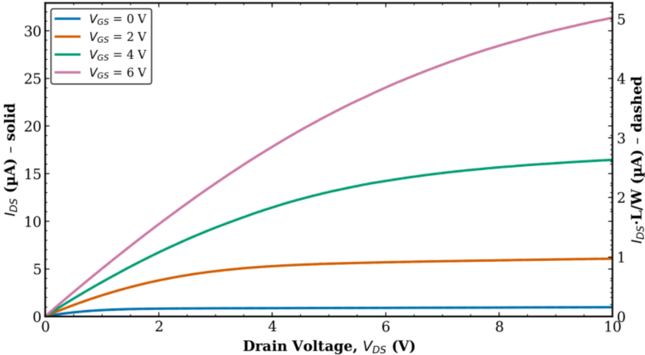
TFT1 Transistor 2 L = 8 \mu\text{m} , W = 50 \mu\text{m}
