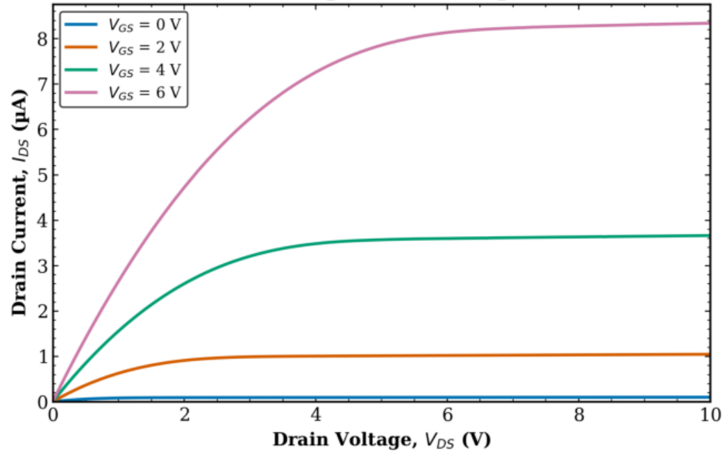
TFT1 Transistor 2 L = 160 \mu\text{m} , W = 100 \mu\text{m}
