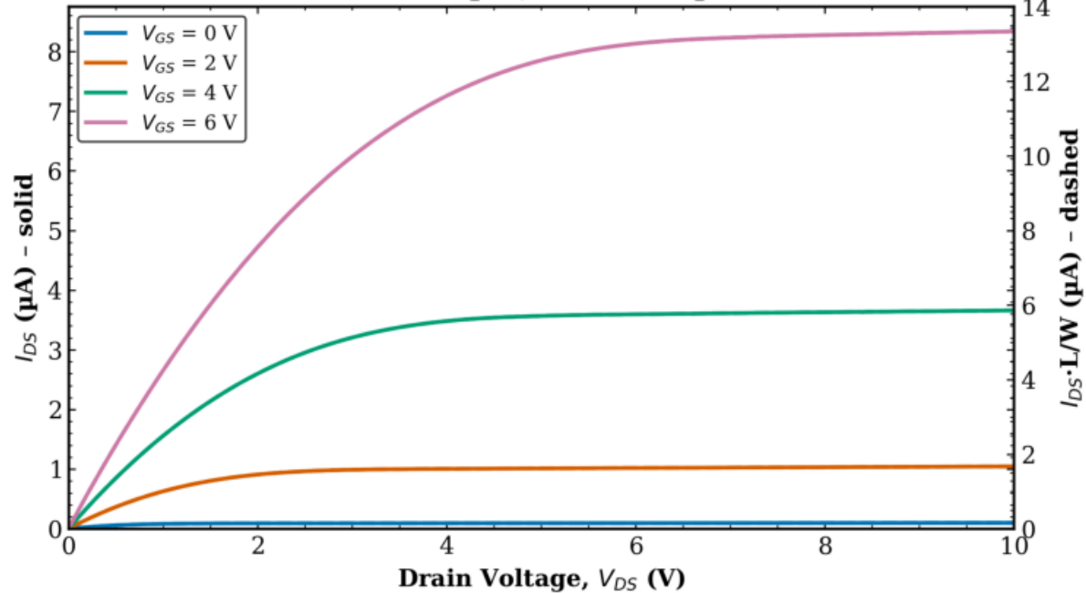
TFT1 Transistor 2 L = 160 \mu\text{m} , W = 100 \mu\text{m}
