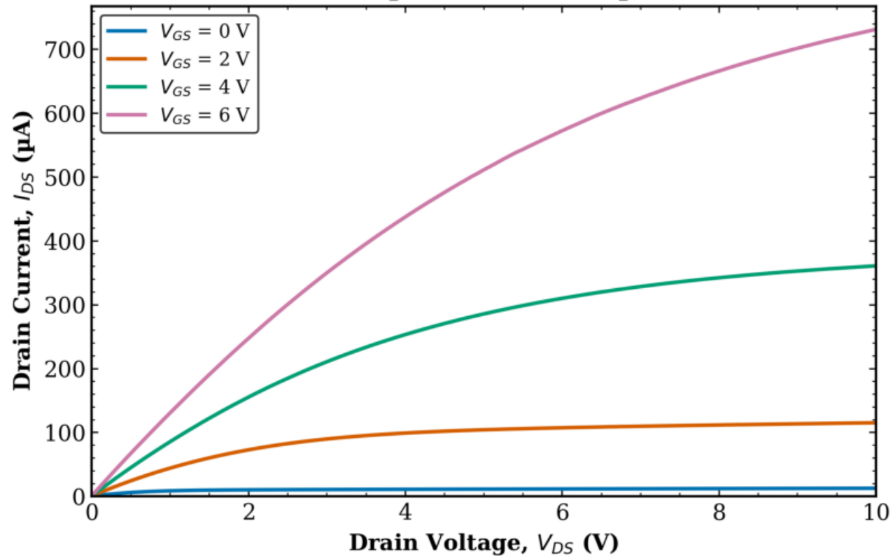
TFT1 Transistor 2 L = 8 \mu\text{m} , W = 1000 \mu\text{m}
