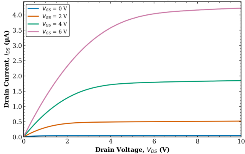
TFT1 Transistor 2 L = 40 \mu\text{m} , W = 10 \mu\text{m}
