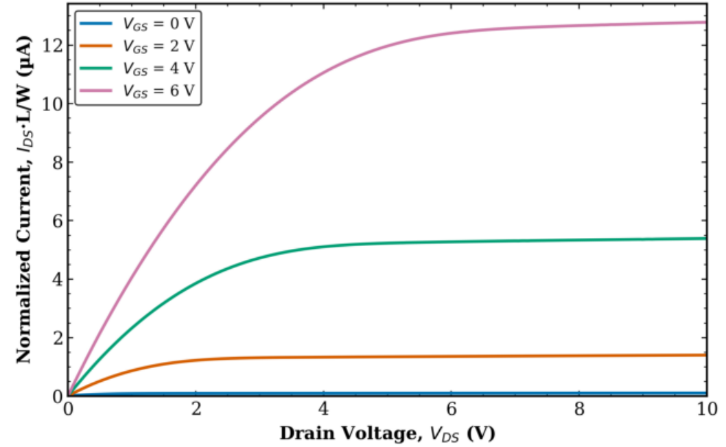
TFT1 Transistor 2 L = 40 \mu\text{m} , W = 100 \mu\text{m} (normalized)
