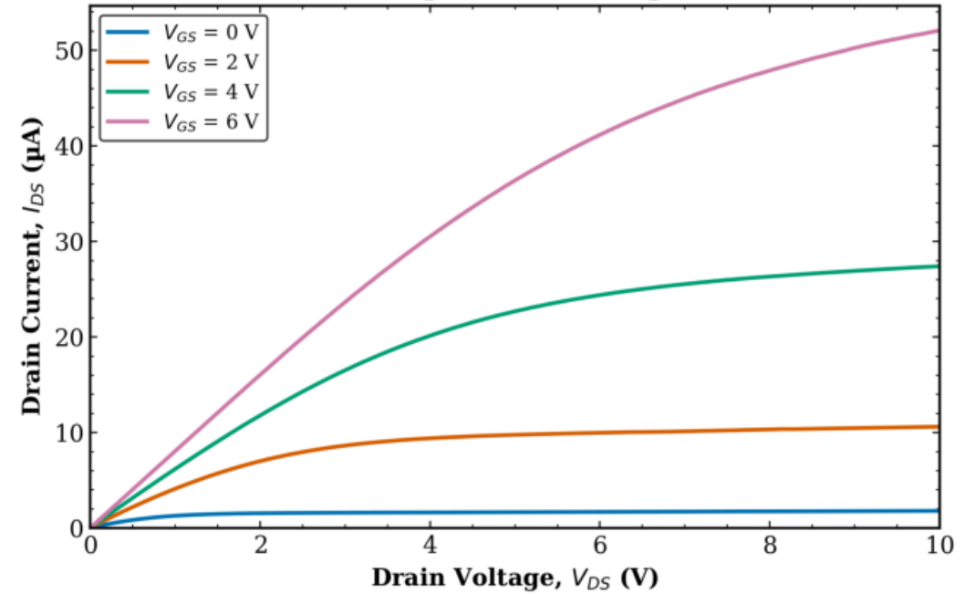
TFT1 Transistor 2 L = 8 \mu\text{m} , W = 100 \mu\text{m}
