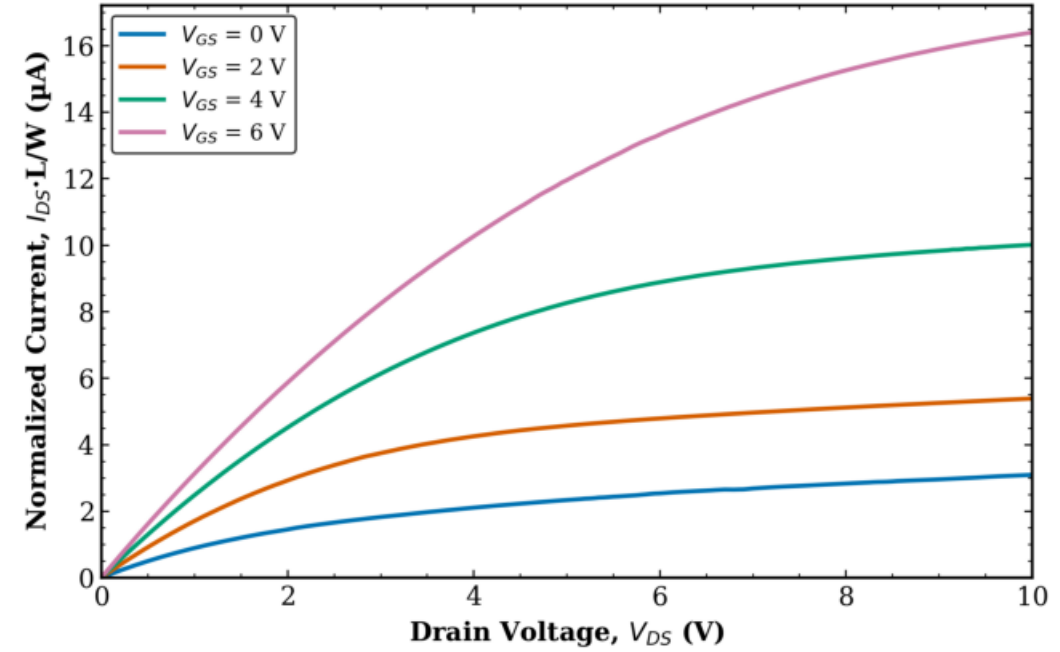
TFT1 Transistor 2 L = 10 \mu\text{m} , W = 100 \mu\text{m} (normalized)
