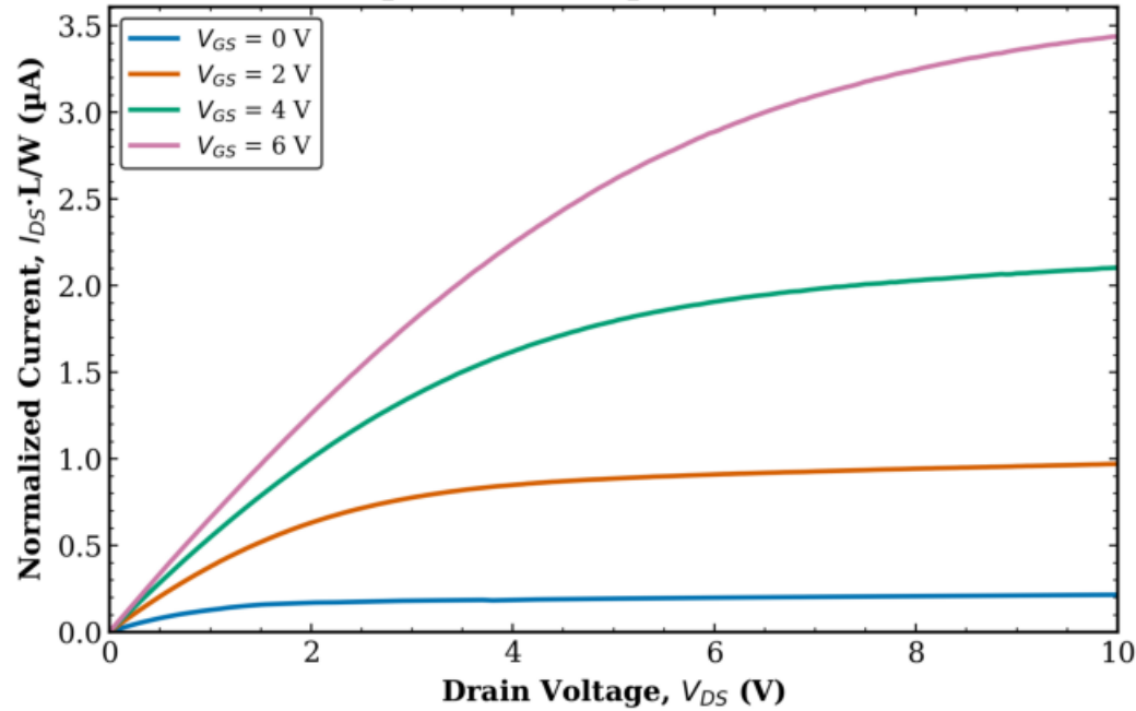
TFT1 Transistor 2 L = 8 \mu\text{m} , W = 10 \mu\text{m} (normalized)
