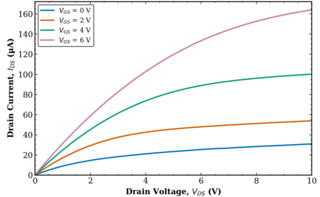
TFT1 Transistor 2 L = 10 \mu\text{m} , W = 100 \mu\text{m}
