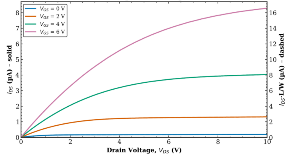
TFT1 Transistor 2 L = 20 \mu\text{m} , W = 10 \mu\text{m}
