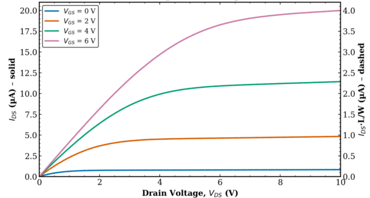
TFT1 Transistor 2 L = 10 \mu\text{m} , W = 50 \mu\text{m}
