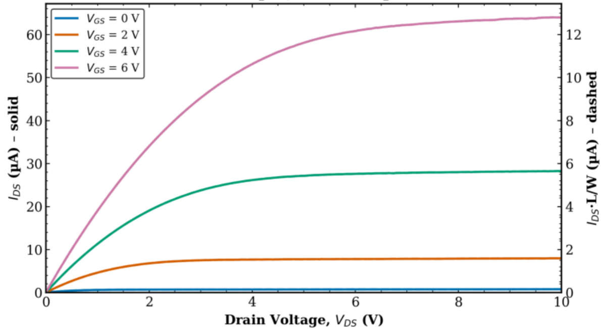
TFT1 Transistor 2 L = 20 \mu\text{m} , W = 100 \mu\text{m}
