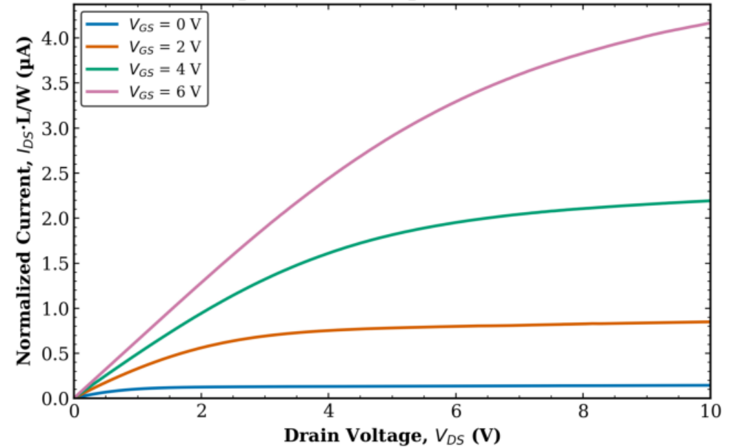
TFT1 Transistor 2 L = 8 \mu\text{m} , W = 100 \mu\text{m} (normalized)
