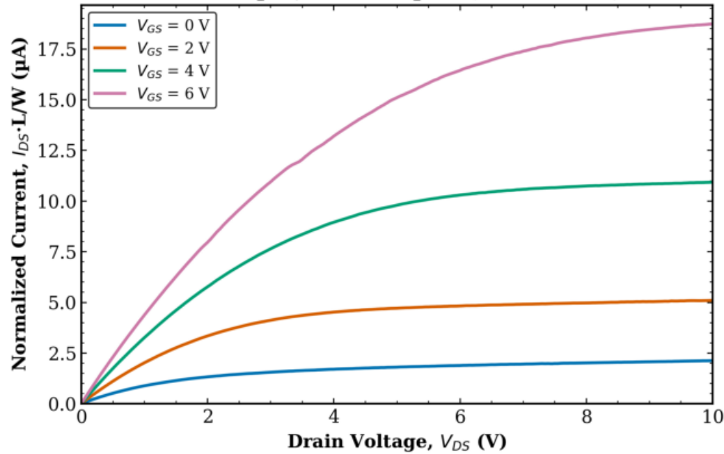
TFT1 Transistor 2 L = 20 \mu\text{m} , W = 50 \mu\text{m} (normalized)
