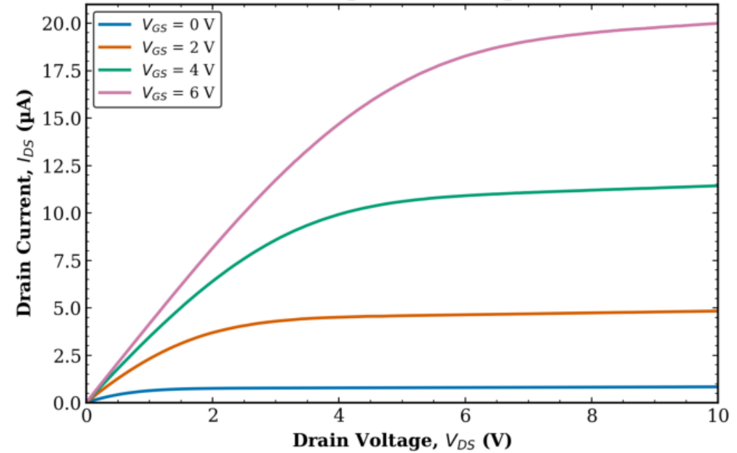
TFT1 Transistor 2 L = 10 \mu\text{m} , W = 50 \mu\text{m}
