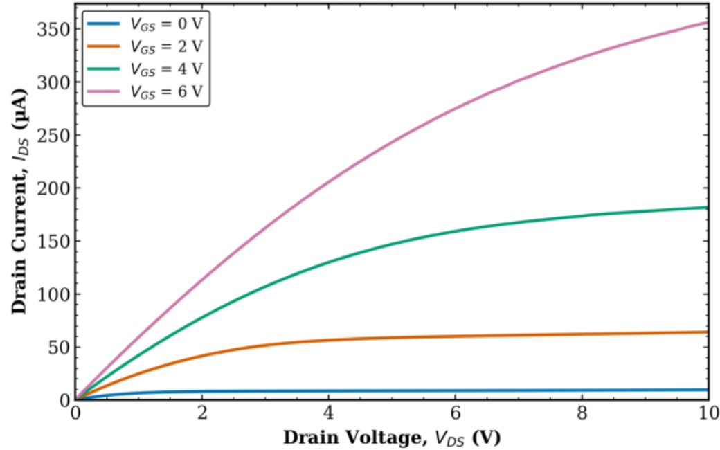
TFT1 Transistor 2 L = 10 \mu\text{m} , W = 500 \mu\text{m}
