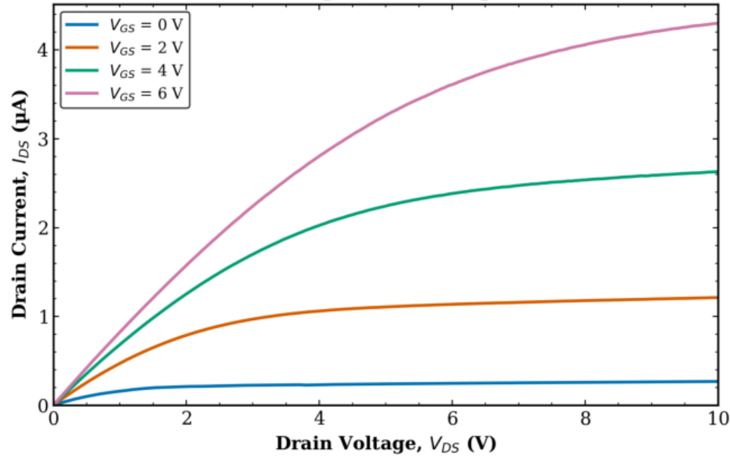
TFT1 Transistor 2 L = 8 \mu\text{m} , W = 10 \mu\text{m}
