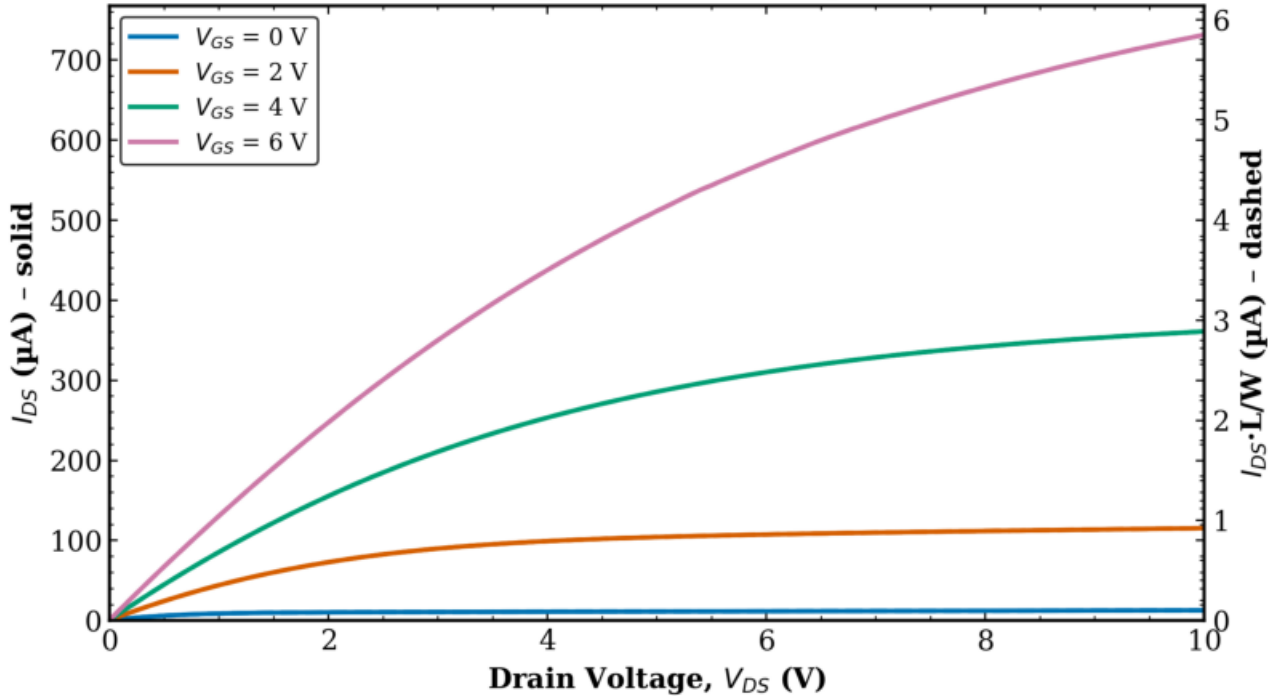
TFT1 Transistor 2 L = 8 \mu\text{m} , W = 1000 \mu\text{m}
