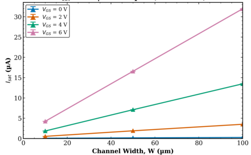
TFT1 Transistor 2 I_{sat} vs W | L = 40 \mu\text{m} (mean \pm std)
