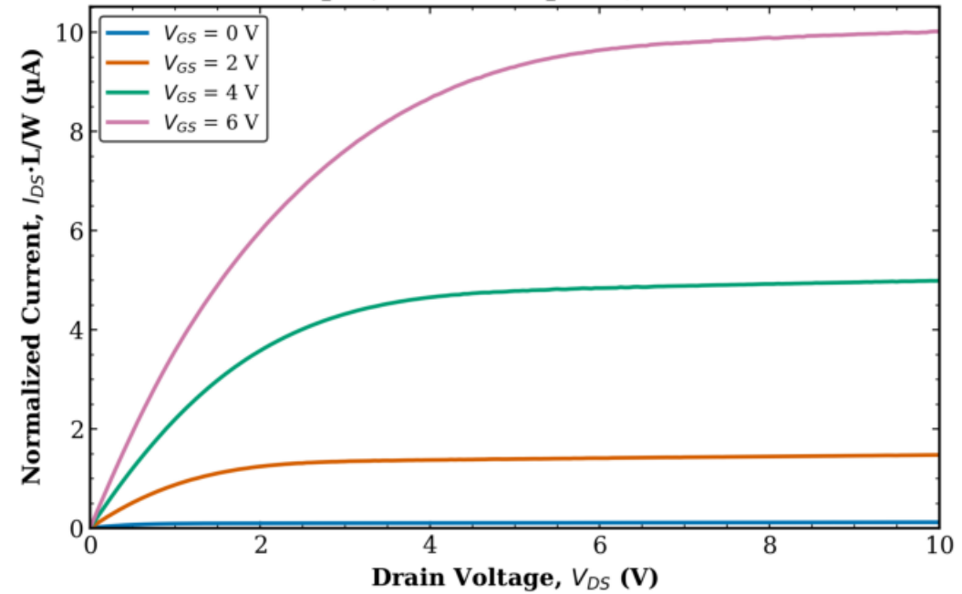
TFT1 Transistor 2 L = 20 \mu\text{m} , W = 500 \mu\text{m} (normalized)
