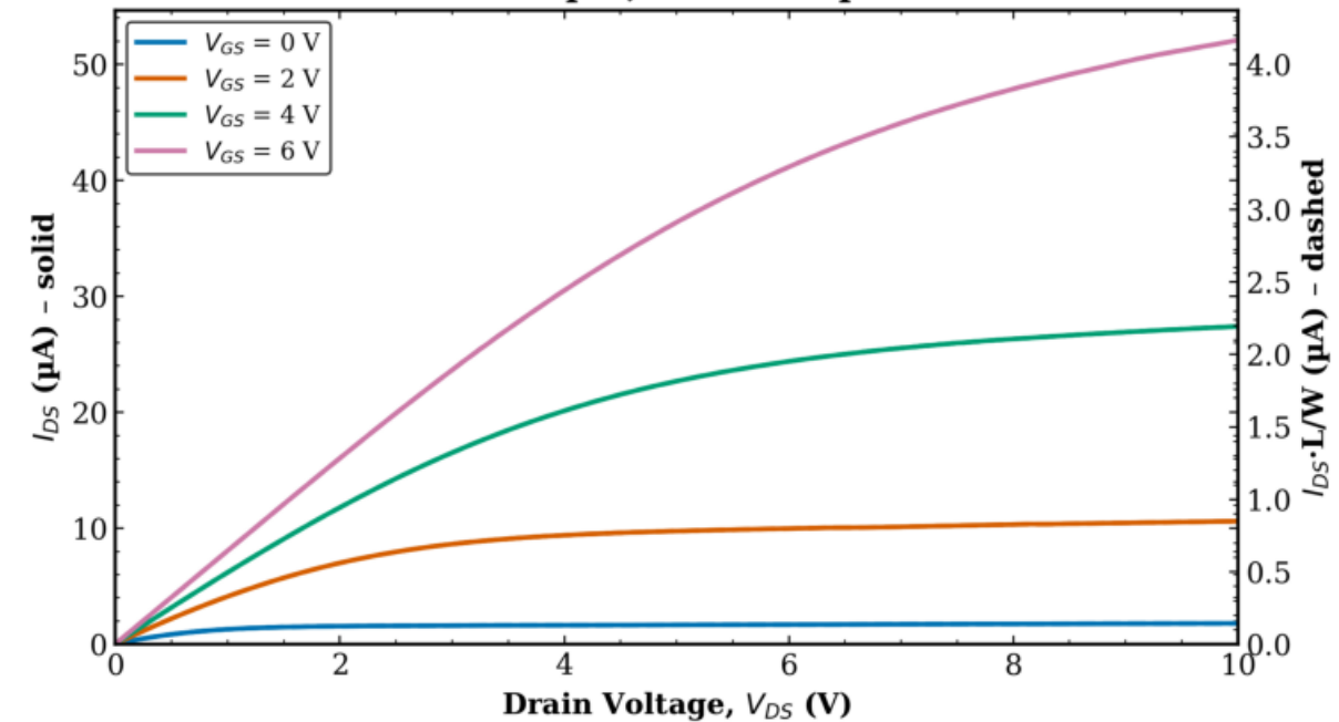
TFT1 Transistor 2 L = 8 \mu\text{m} , W = 100 \mu\text{m}
