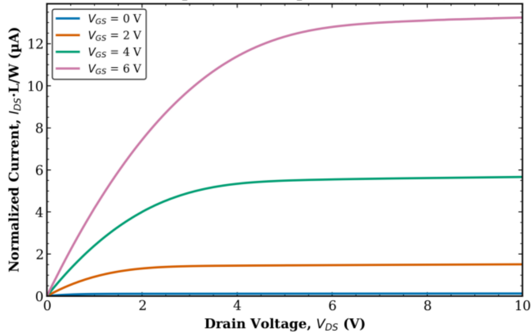
TFT1 Transistor 2 L = 40 \mu\text{m} , W = 50 \mu\text{m} (normalized)
