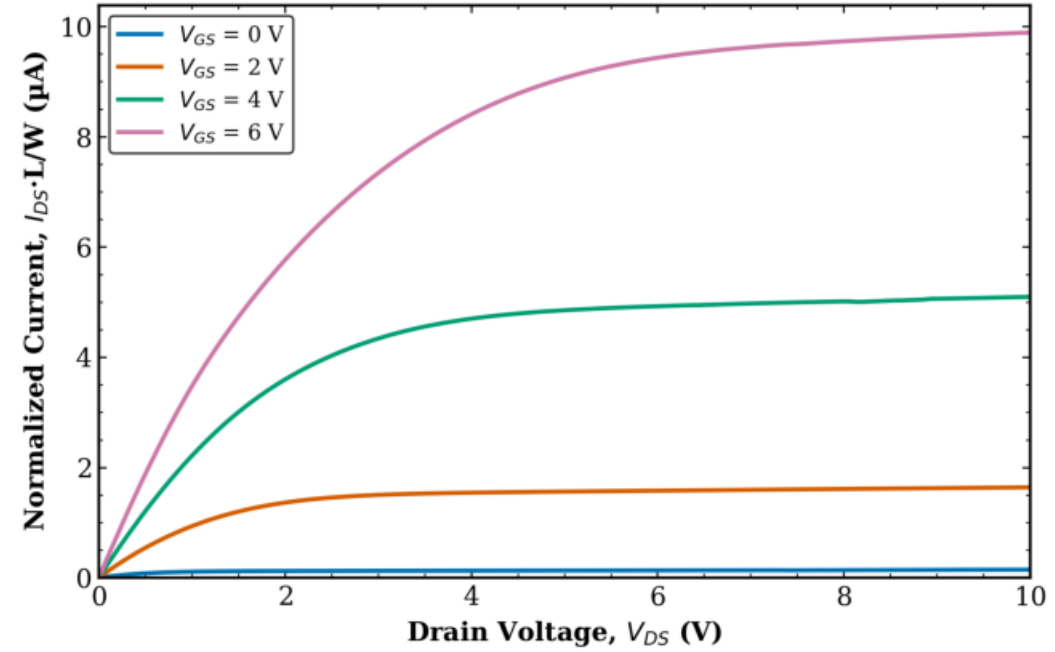
TFT1 Transistor 2 L = 20 \mu\text{m} , W = 1000 \mu\text{m} (normalized)
