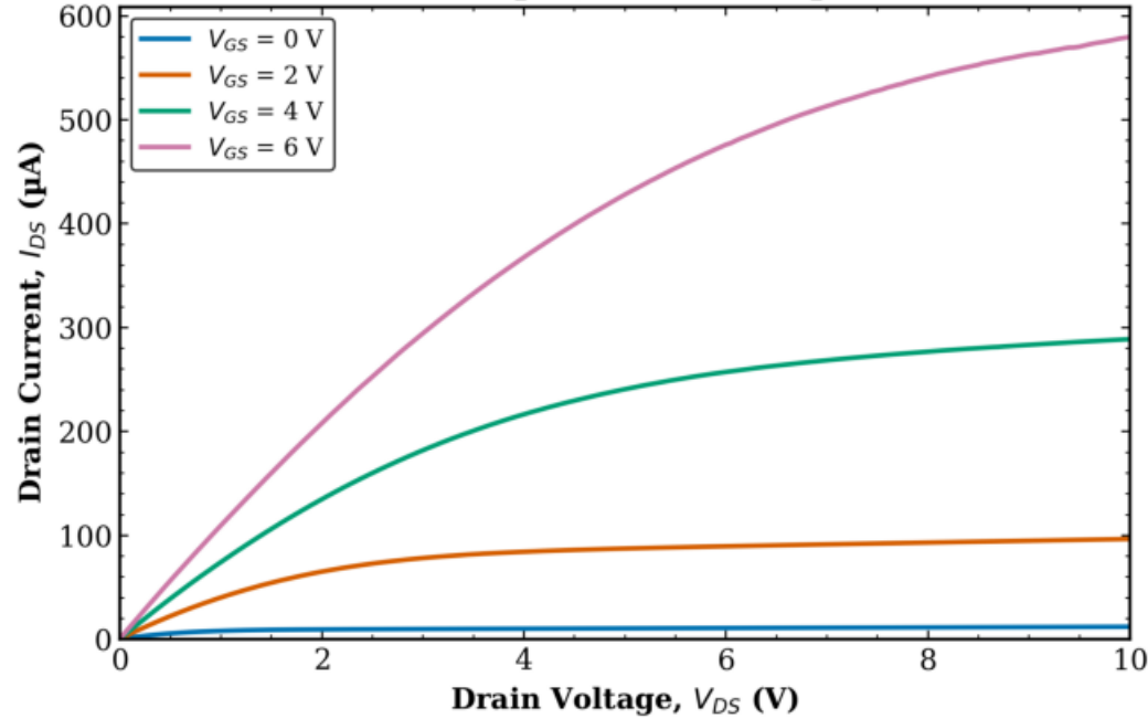
TFT1 Transistor 2 L = 10 \mu\text{m} , W = 1000 \mu\text{m}
