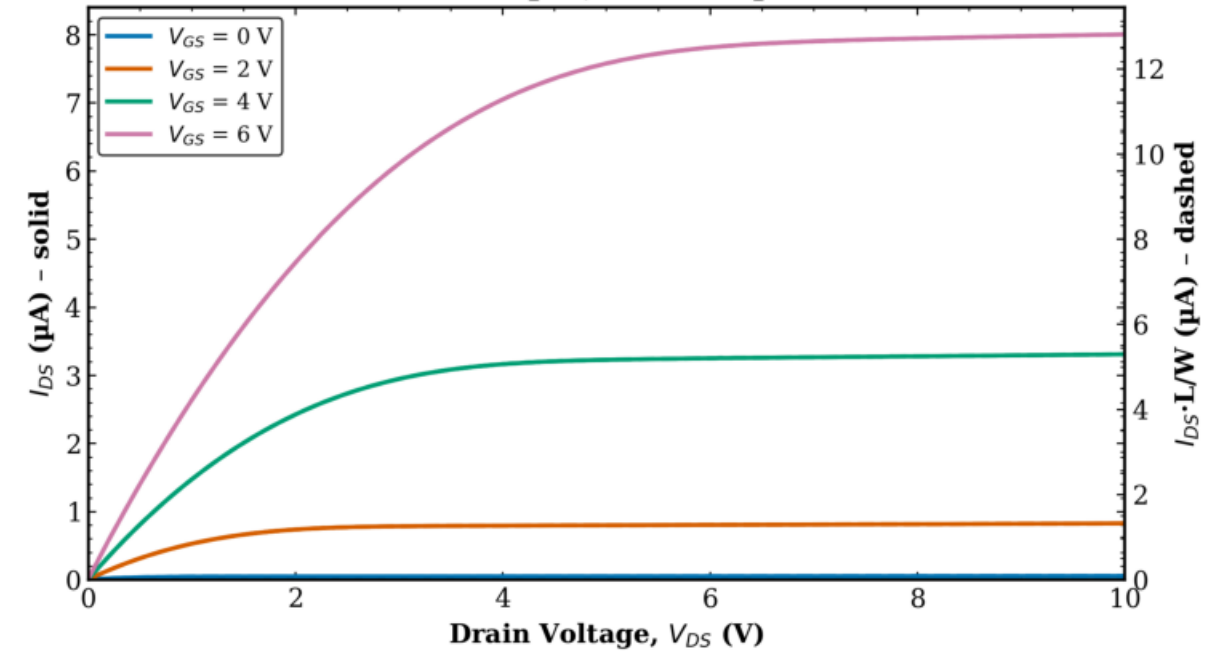
TFT1 Transistor 2 L = 80 \mu\text{m} , W = 50 \mu\text{m}
