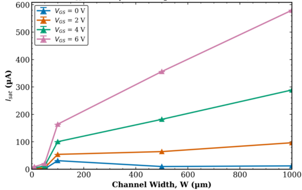
TFT1 Transistor 2 I_{sat} vs W | L = 10 \mu\text{m} (mean \pm std)
