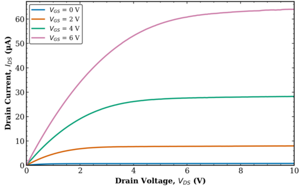
TFT1 Transistor 2 L = 20 \mu\text{m} , W = 100 \mu\text{m}
